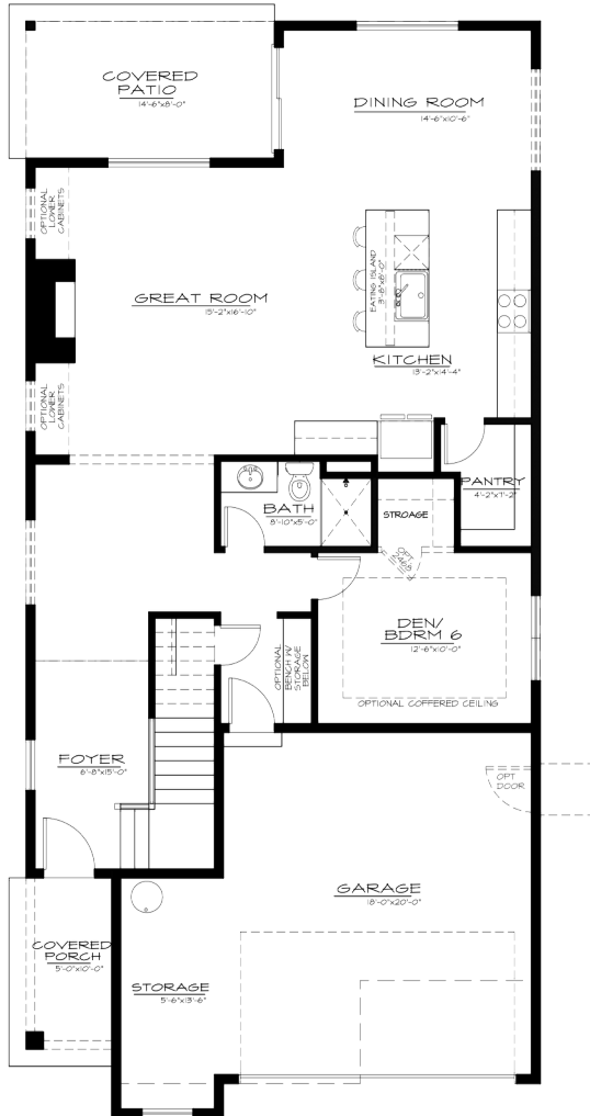
1ST FLOOR
