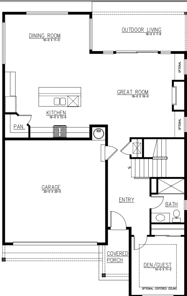
1ST FLOOR
